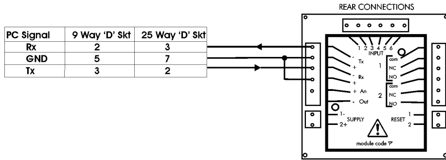
Figure 7.3 RS232 Mode to PC
