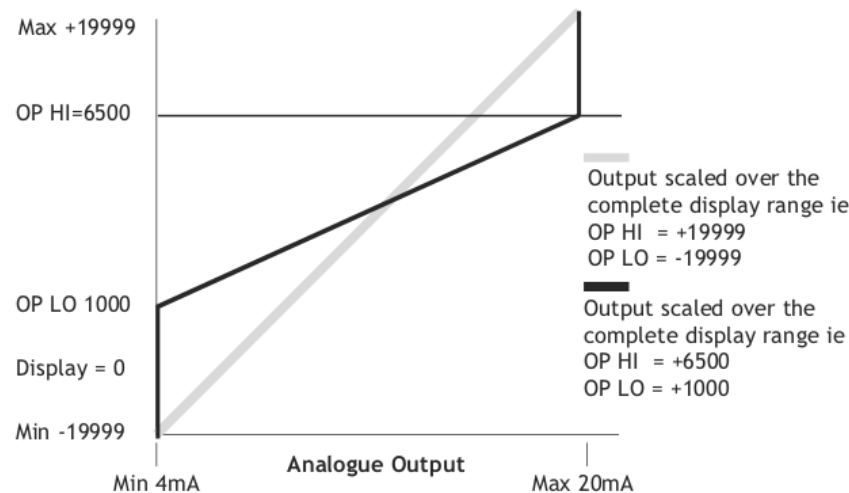
Figure 6.1 Analogue Output
