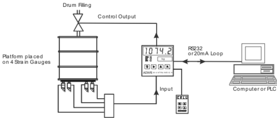
Figure 1.2 Drum Filling
