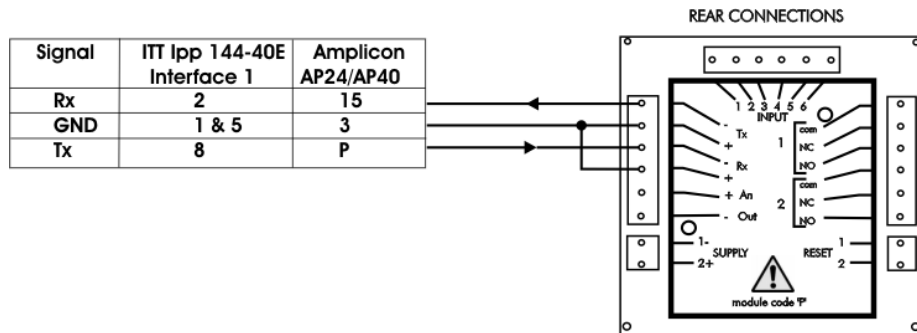
Figure 7.4 RS232 Mode to Printer
